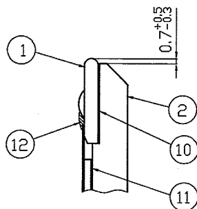
MAGNIFIED VIEW OF PART "A" (2/1)
