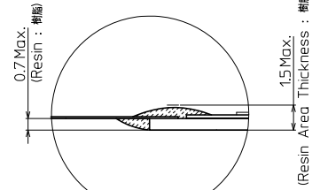
DETAIL D (5:1)
