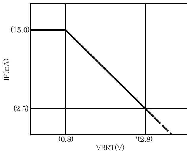
VBRT-IF characteristics (reference) T_a = 25^\circ C
